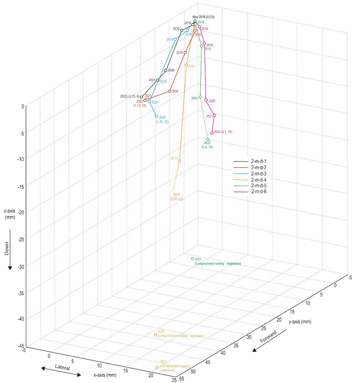
FIGURE 17- AREA 2, LINE D, 3D GRAPH OF X,Y,Z MOVEMENT OVER DURATION OF THE MONITORING SURVEY OF EACH SURVEY MARKER.
