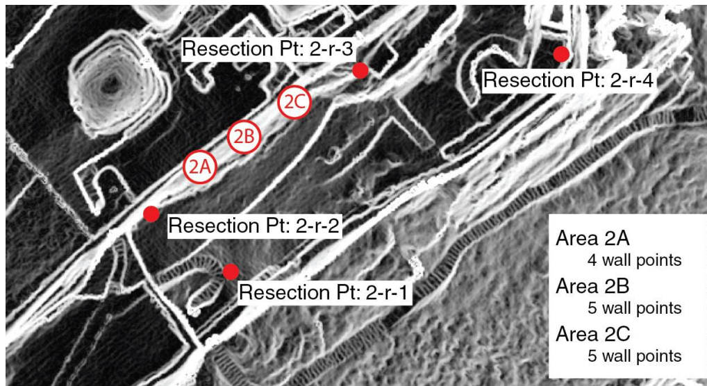
FIGURE III - PLAN LOCATING RESECTION CONTROL NETWORK FOR AREA 2
