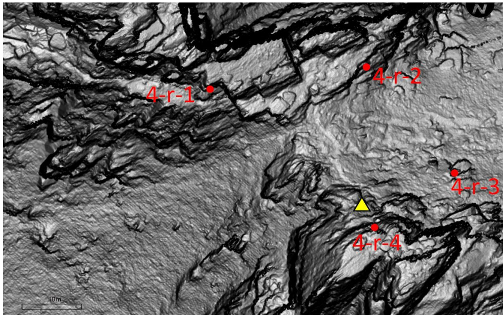
FIGURE VII - PLAN LOCATING RESECTION CONTROL NETWORK FOR AREA 4
