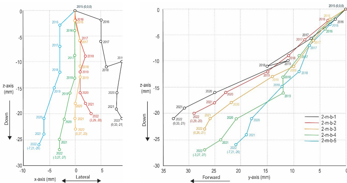
FIGURE 14 - AREA 2, LINE B, LATERAL AND FORWARD MOVEMENT 2D GRAPHS
