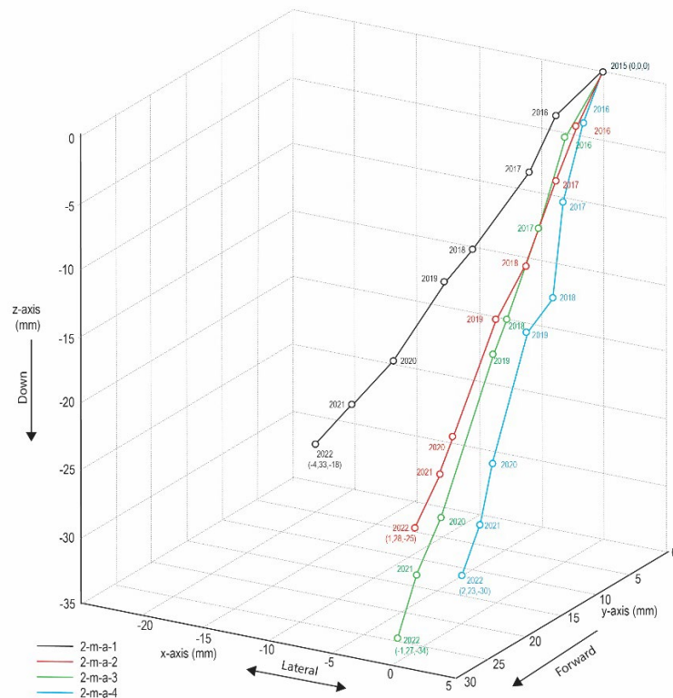
FIGURE 11 - AREA 2, LINE A, 3D GRAPH OF x,y,z MOVEMENT OVER DURATION OF THE MONITORING SURVEY OF EACH SURVEY MARKER
