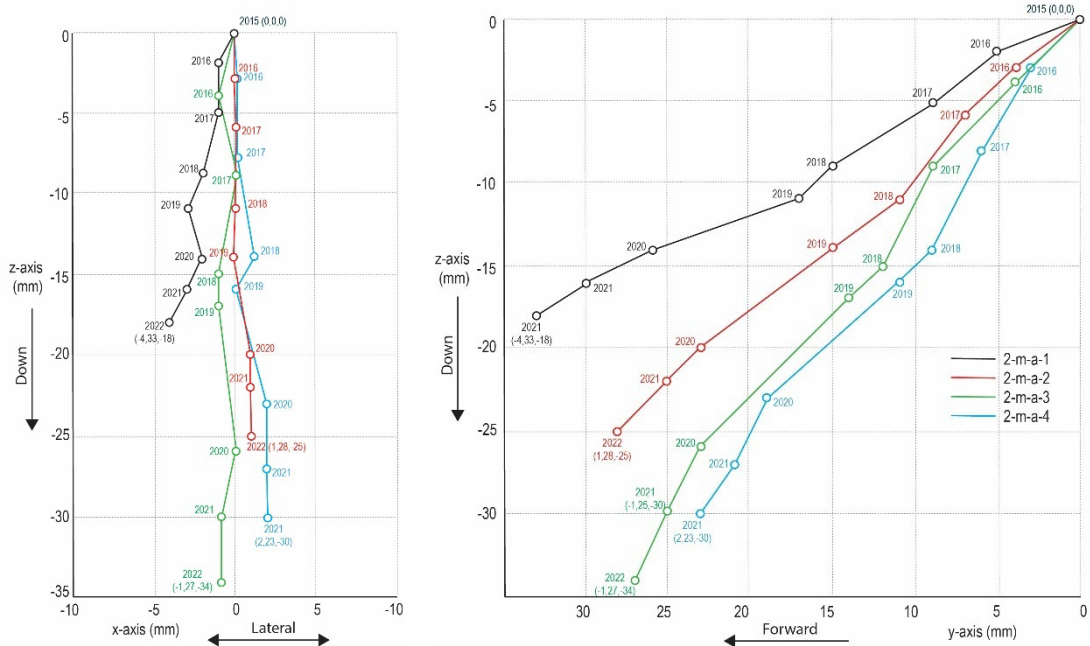
FIGURE 12 – AREA 2, LINE A, LATERAL AND FORWARD MOVEMENT 2D GRAPHS
