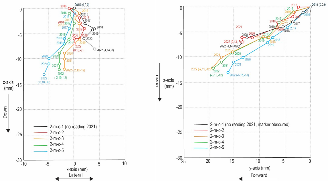
FIGURE 16 - AREA 2, LINE C, LATERAL AND FORWARD MOVEMENT 2D
