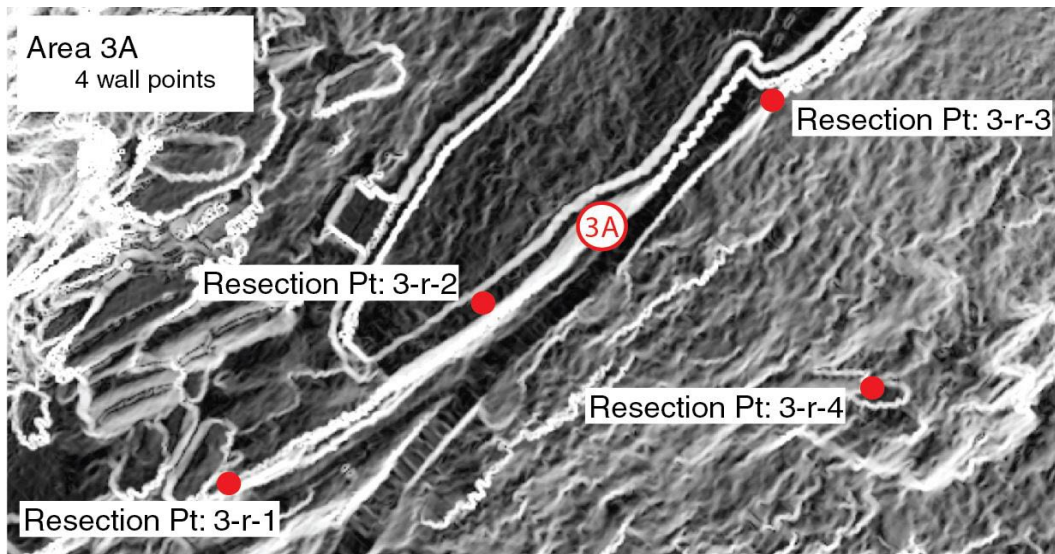
FIGURE V - PLAN LOCATING RESECTION CONTROL NETWORK FOR AREA 3
