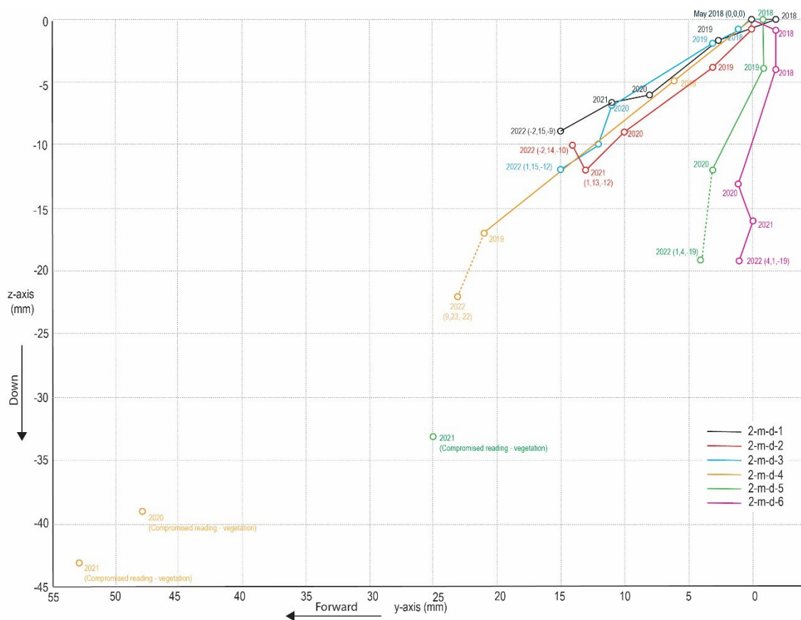
FIGURE 18 - AREA 2, LINE D, LATERAL AND FORWARD MOVEMENT 2D
