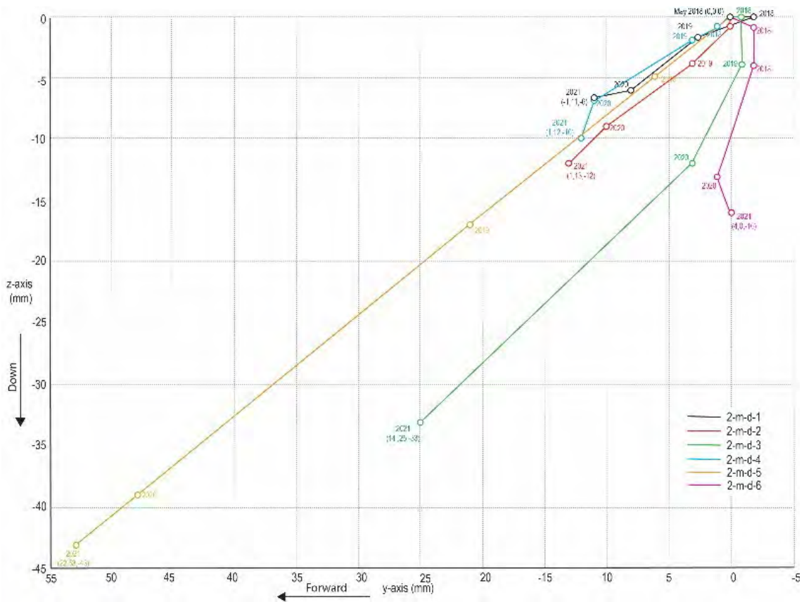
FIGURE 18 - AREA 2, LINE D, LATERAL AND FORWARD MOVEMENT 2D
