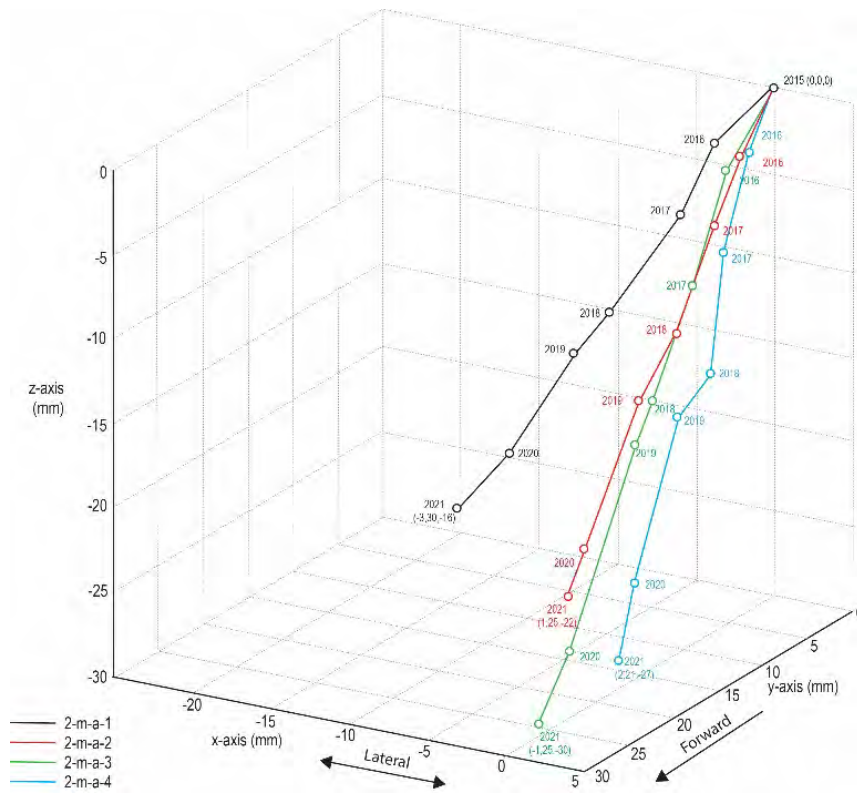
FIGURE 11 - AREA 2, LINE A, 3D GRAPH OF X,Y,Z MOVEMENT OVER DURATION OF THE MONITORING SURVEY OF EACH SURVEY MARKER
