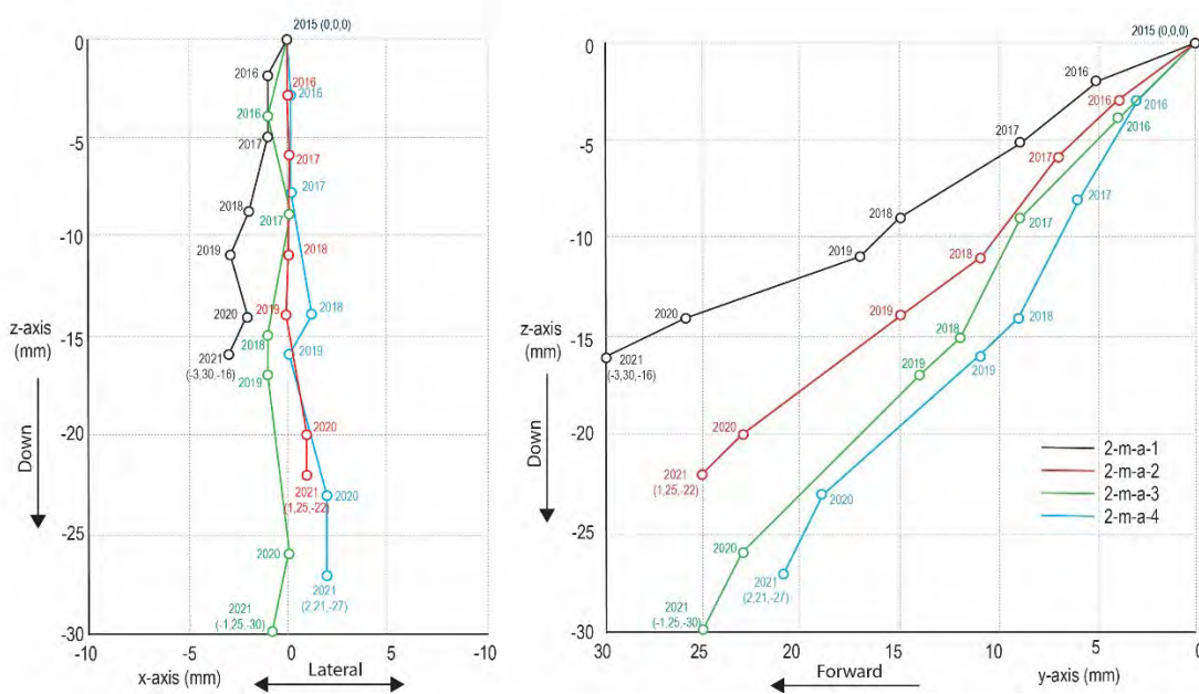
FIGURE 12 – AREA 2, LINE A, LATERAL AND FORWARD MOVEMENT 2D GRAPHS
