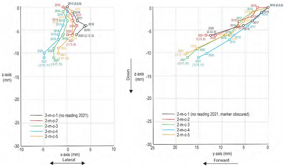
FIGURE 16 - AREA 2, LINE C, LATERAL AND FORWARD MOVEMENT 2D
