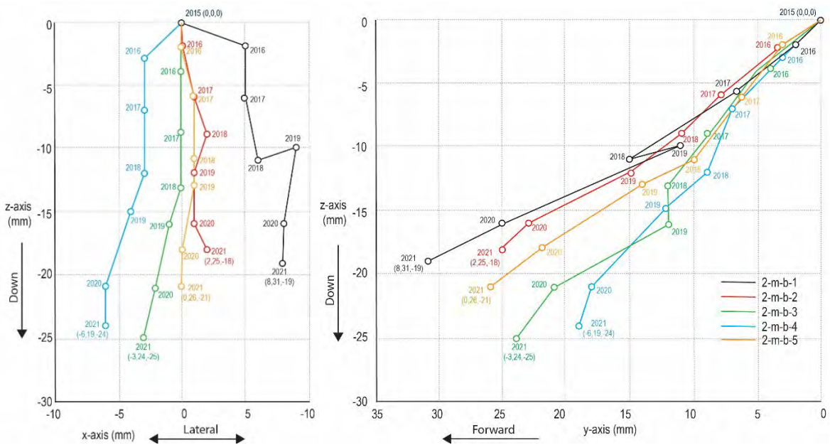
FIGURE 14 - AREA 2, LINE B, LATERAL AND FORWARD MOVEMENT 2D GRAPHS
